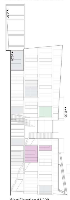
West Elevation #1:200
