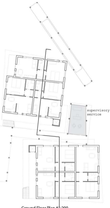
Ground Floor Plan #1:200
